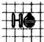
HOOH
